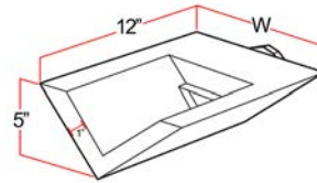
V-Shaped Scupper
