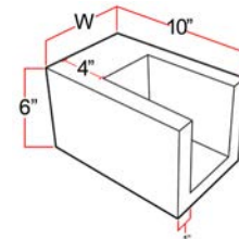
U-Shaped Scupper
