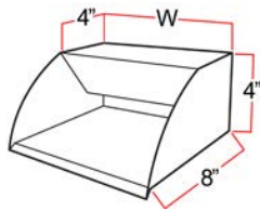
Radius Scupper
