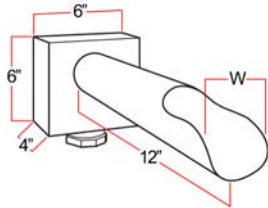
Cannon Scupper
