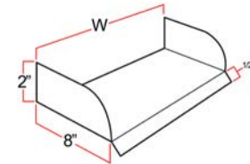
Straight Spillway
